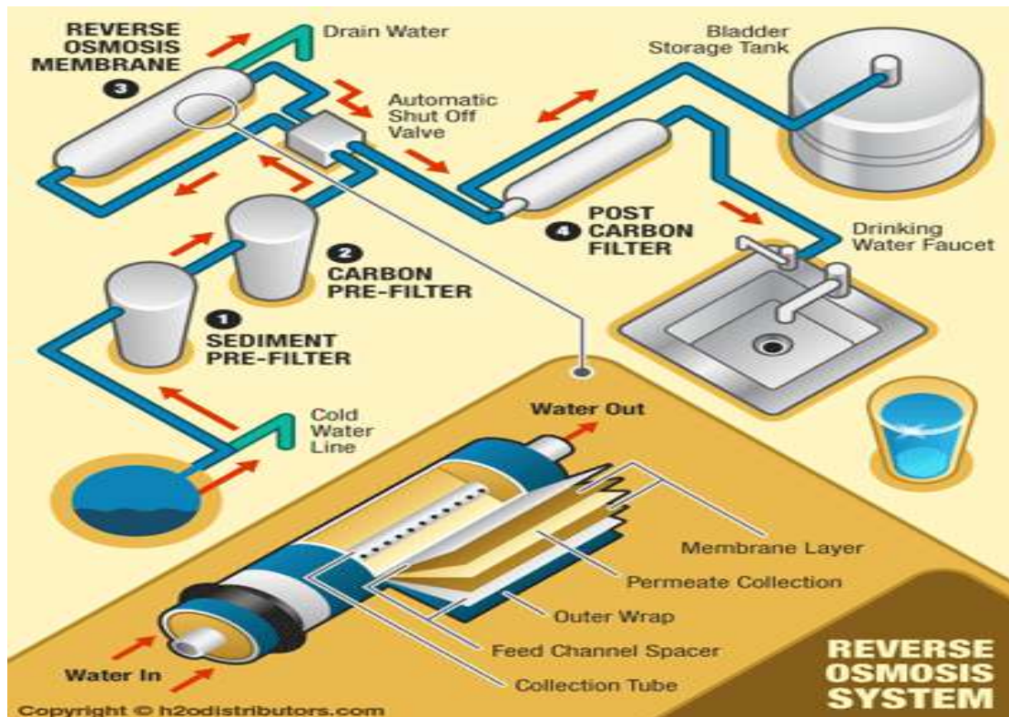
Figure 2.1: Over view reverse osmosis system
