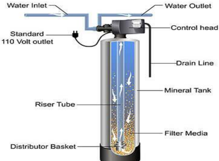
Carbon tank filtration systems(B)
