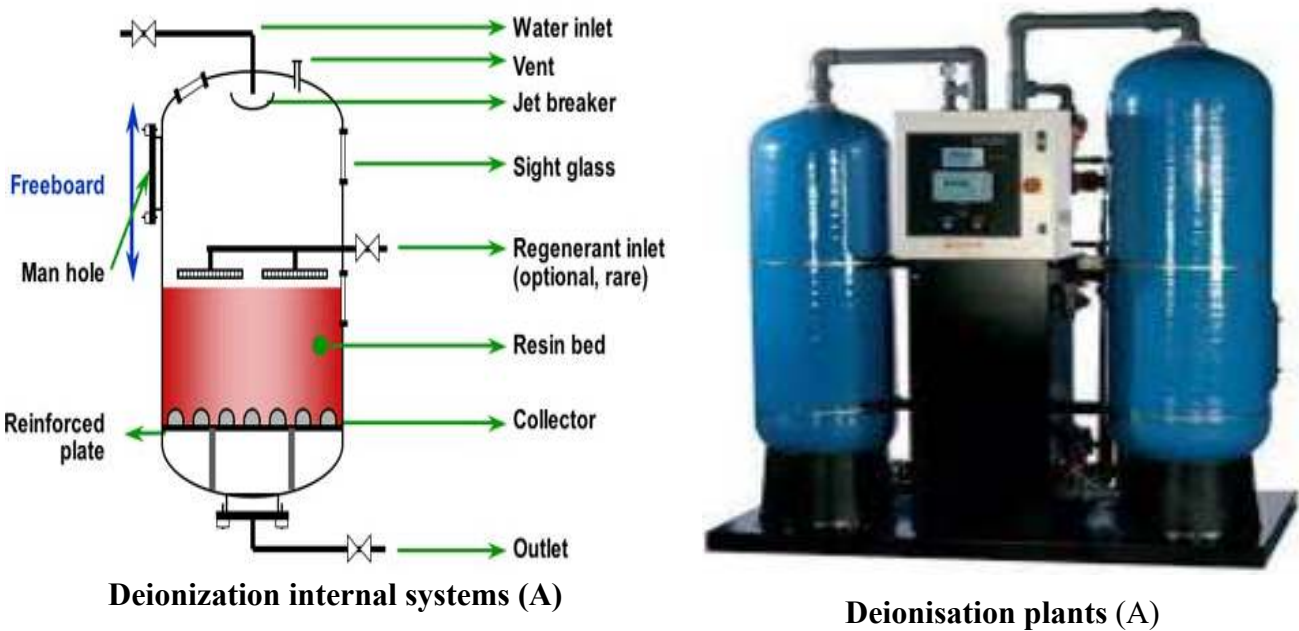
Figure 1.6: Deionisation plants
