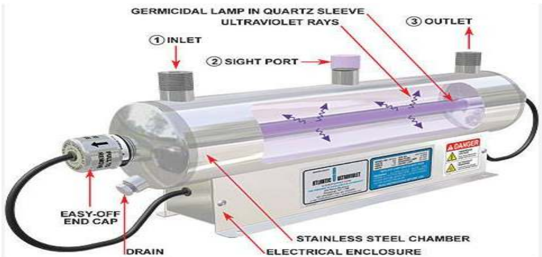
Figure 1.5: UV lighter
