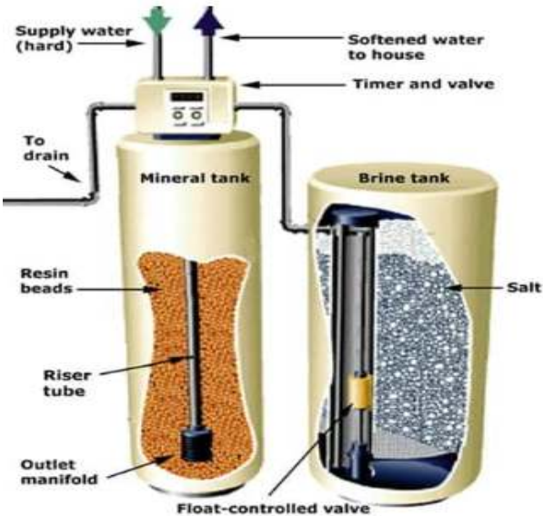
Softener internal system(A)
