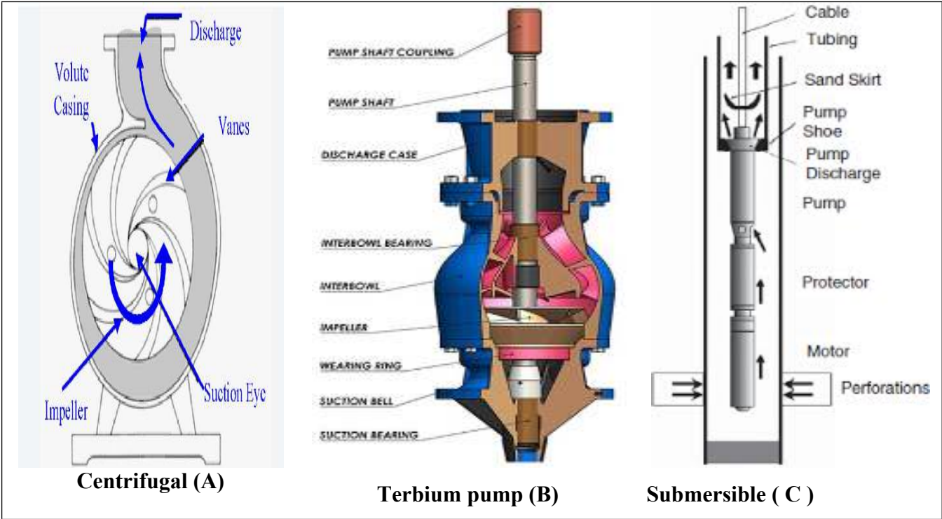
Figure 1.3: Water pumper
