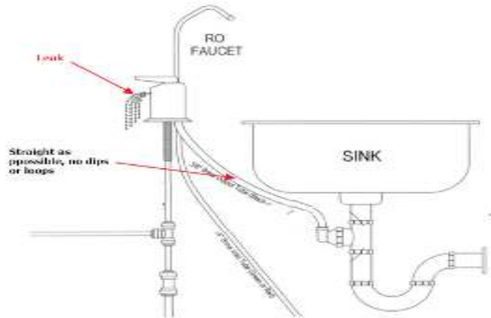
Figure 2.3: Faucet system
